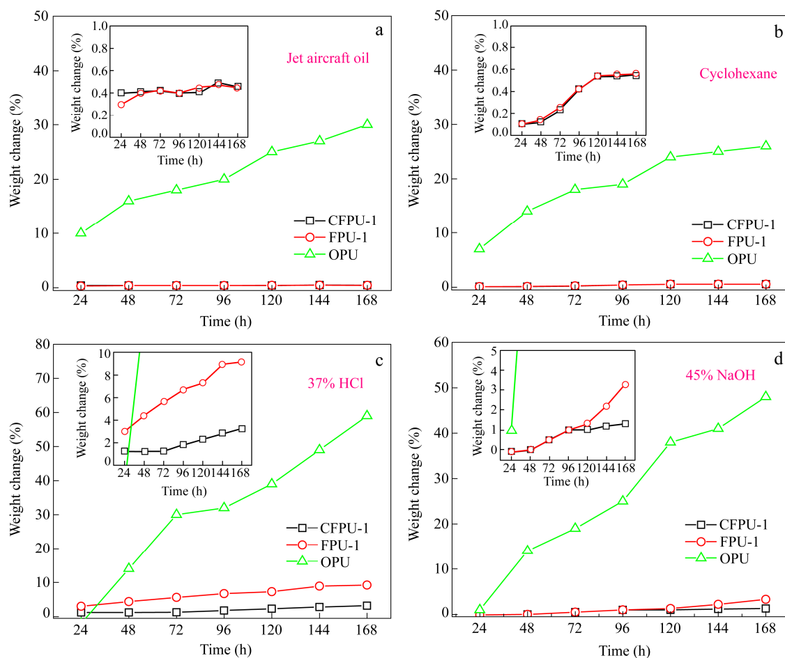
Fig. 12 Weight change of CFPU-1, FPU-1 and OPU films in four different solutions: Jet aircraft oil (a), cyclohexane (b), 37% HCl (c) and 45% NaOH (d) at different time at room temperature (The insets show the amplified corresponding graphs.)
